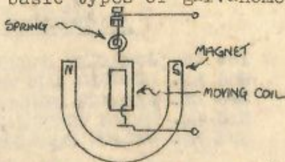
Fig. 100(b) Fixed Magnet-Moving Coil Type of Galvanometer
