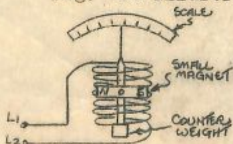
Fig. 100(a) Fixed Coil-Moving Magnet Type of Galvanometer
